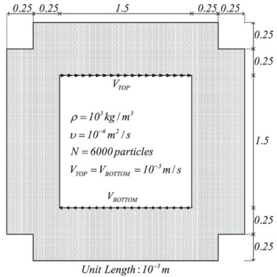
Fig. 22. Holed corner-cut 2D shear driven cavity problem.
