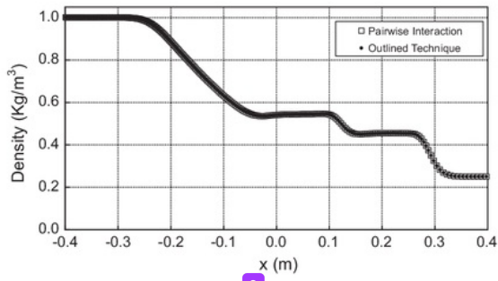
Fig. 4. Density distribution in the shock tube at t = 0.20 s.
