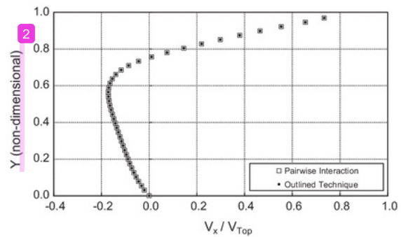
Fig. 10. Horizontal velocities distribution along the vertical centerline.
