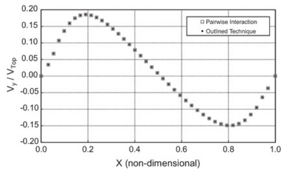
Fig. 9. Vertical velocities distribution along the horizontal centerline.
